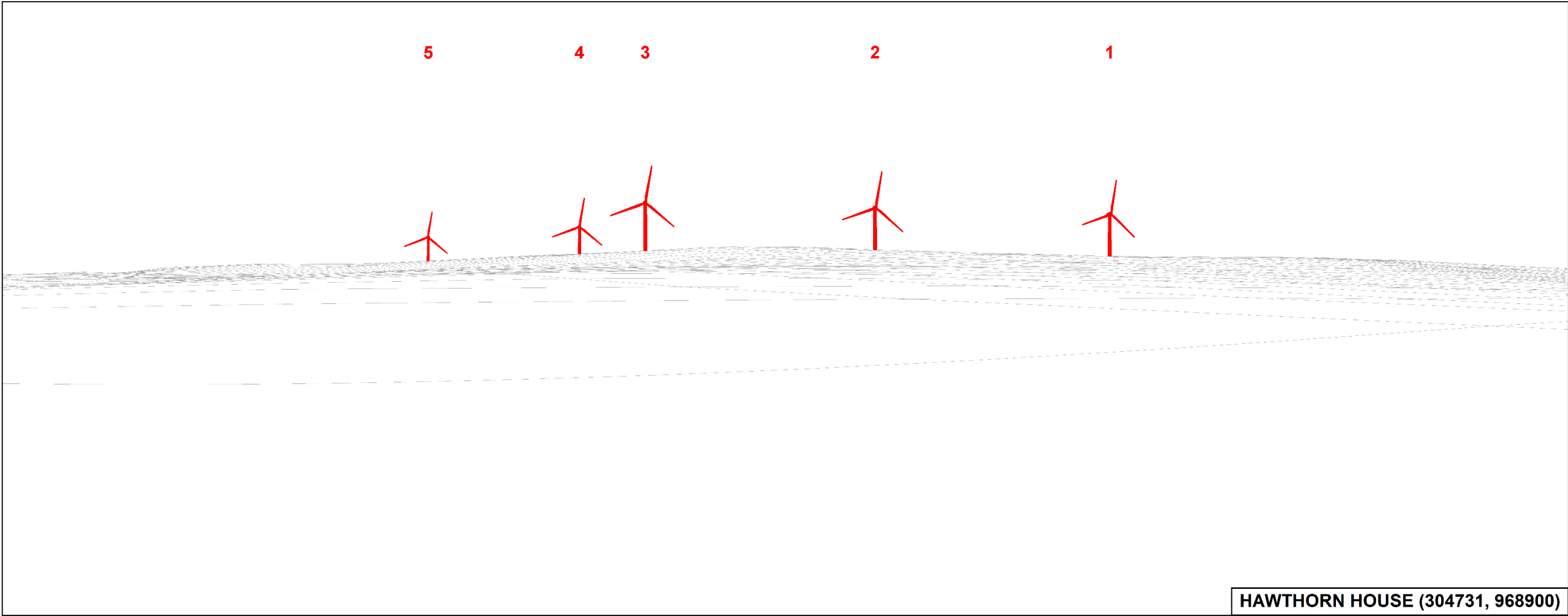
Figure 3.2 - Additional (90 degree) wireline from Hawthorn House (Property Group 2) - based on layout PSCOhof060
